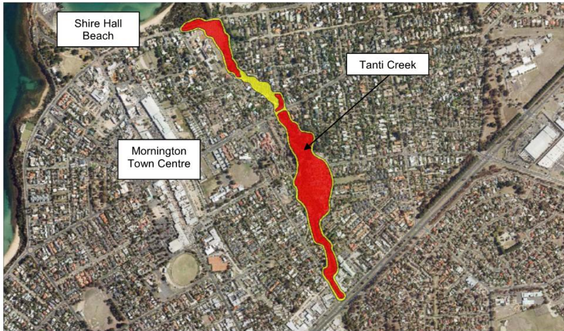
Figure 7-2: Tanti Creek Landslide Susceptibility Zones
