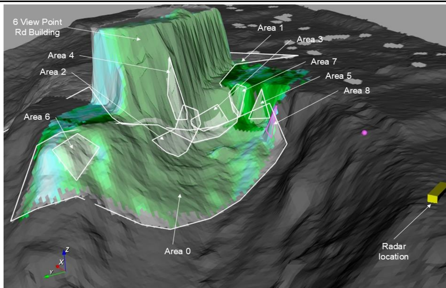
Hardwood Andrews McCrae Landslide Incident Instrumentation and Monitoring Radar - Monitoring Areas
