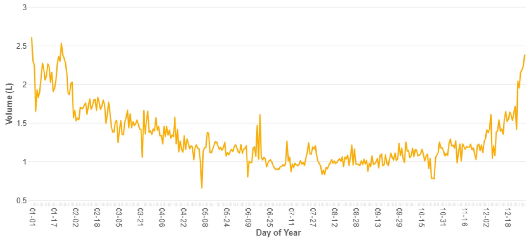
Figure 5: Profile of a typical year for the balance of water usage in the McCrae metered area
