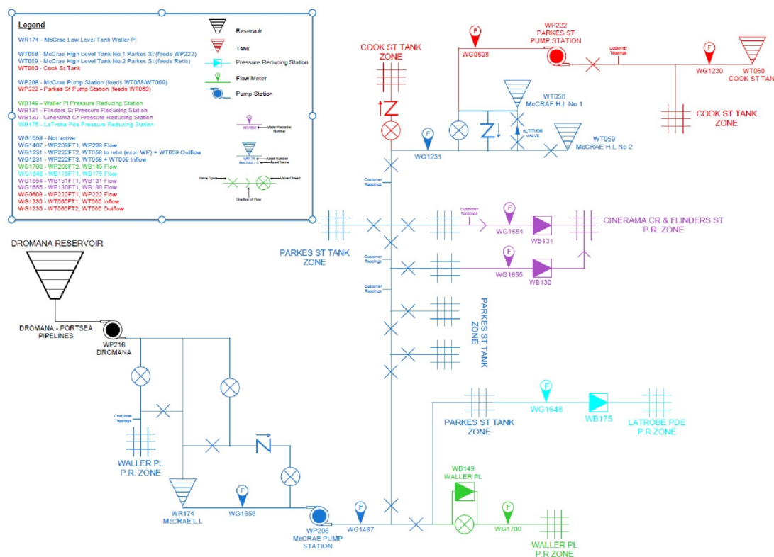
Figure 1: McCrae network zone and monitoring stations
