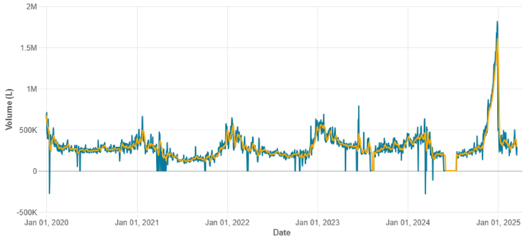
Figure 4: Water balance for the McCrae area (blue) and 7-day rolling average (yellow)
