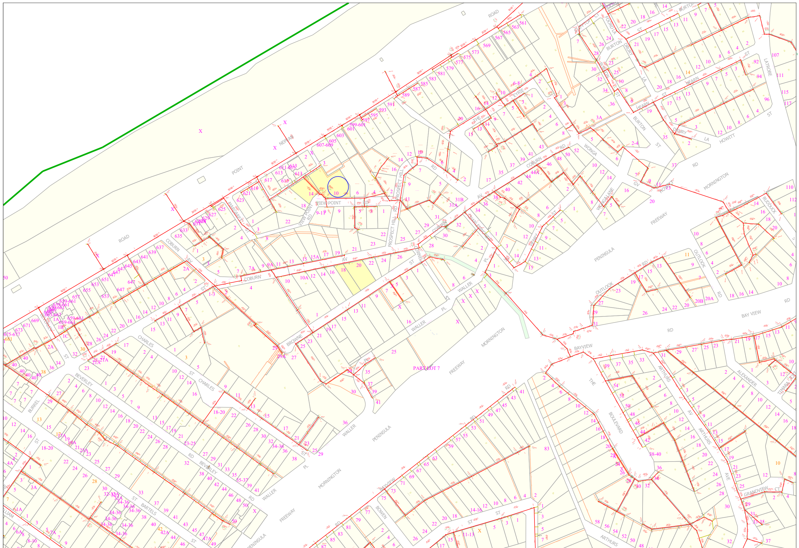
Appendix 2: Plan showing sewerage network around vicinity of the Landslide site. The blue circle shows the location of the Landslide.
