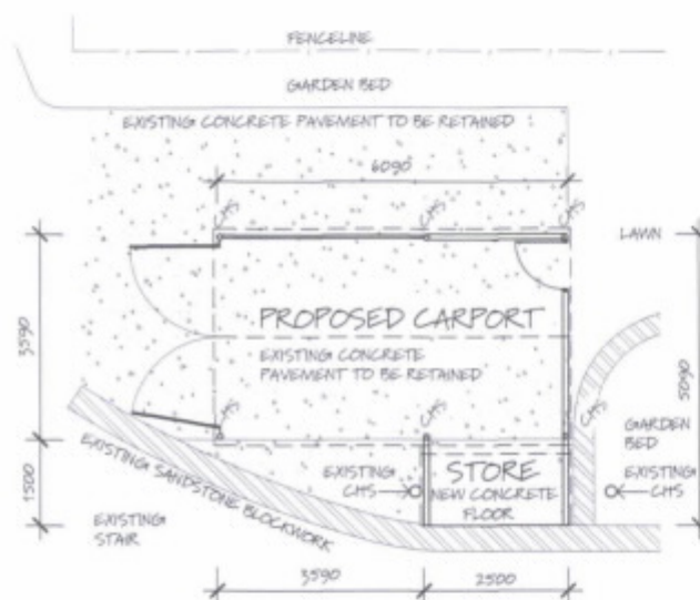
FLOORPLAN SCALE 1:100 AREA = 25.6sqm
